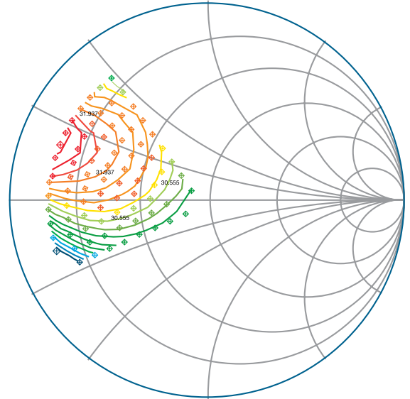
Example of load pull measurements with Output Power (Pout) contours plotted on a Smith Chart.
